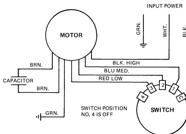
M2500 WIRING DIAGRAM
