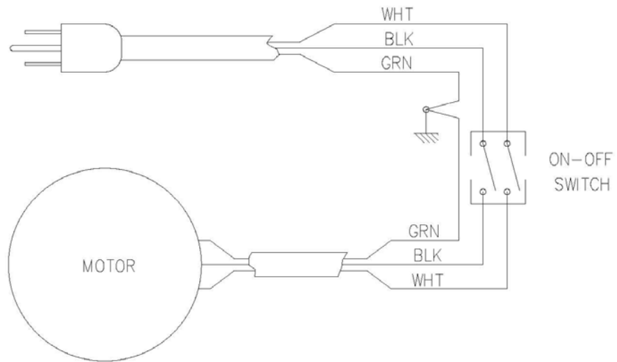
WIRING DIAGRAM
