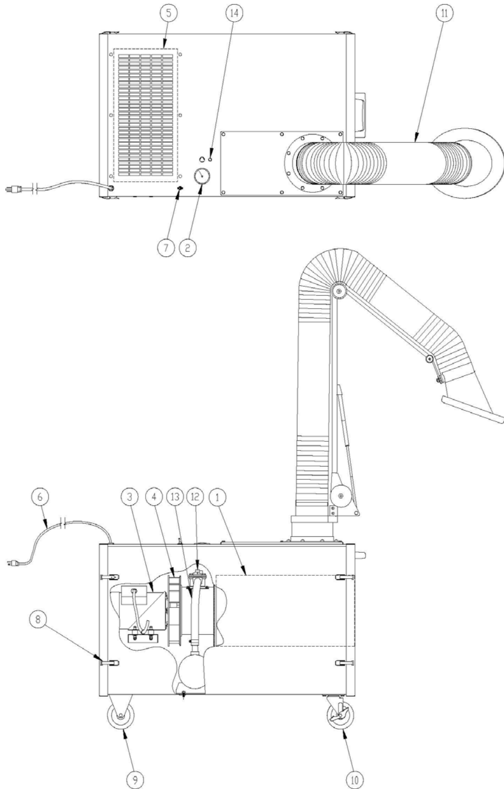
Figure 3-Parts List Diagram
